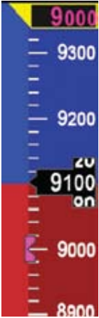
Figure 2-31 Altitude Tape
